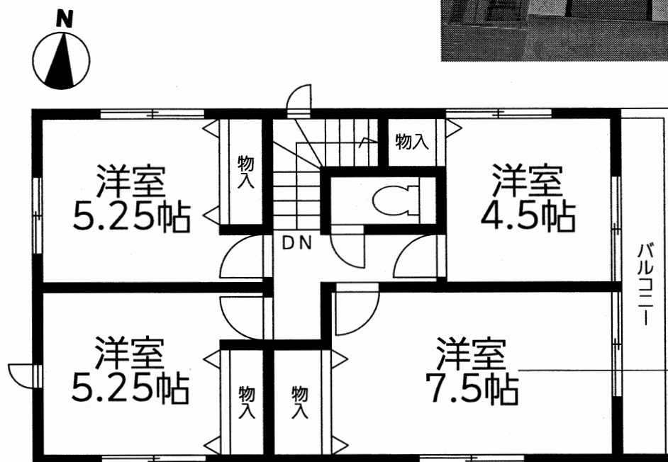
2階平面図:49.68㎡(15.02坪)
