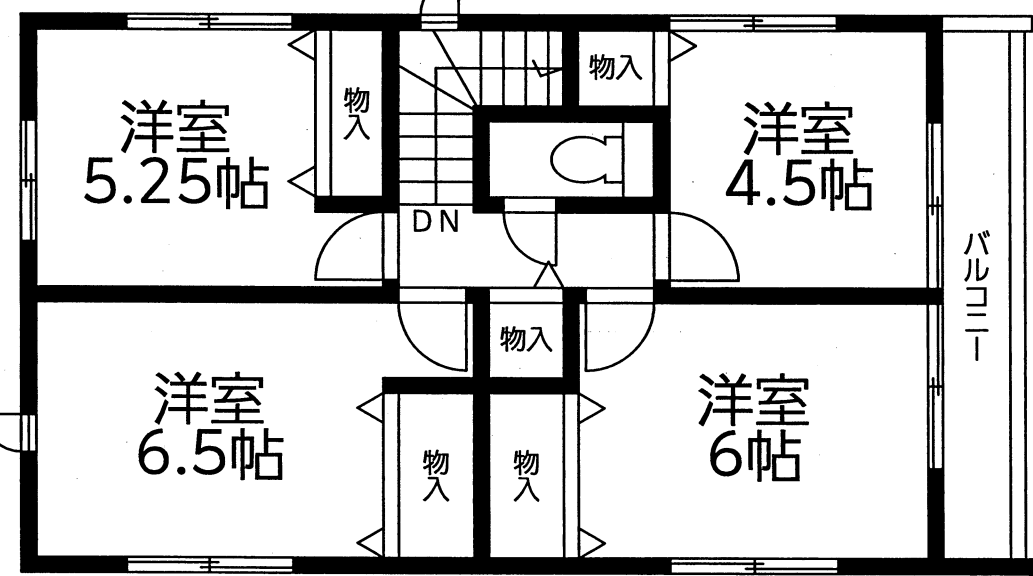
2階平面図:49.68㎡(15.02坪)
